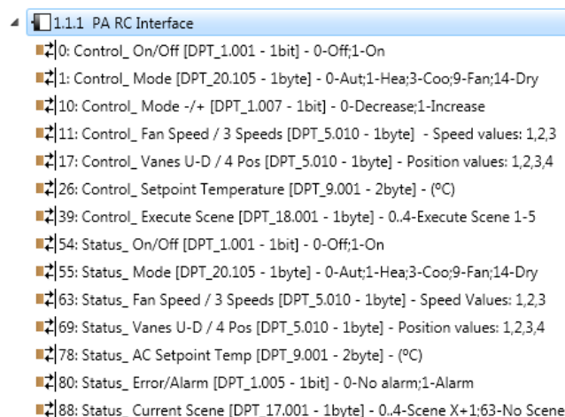
Figure 4.2 Default communication objects
